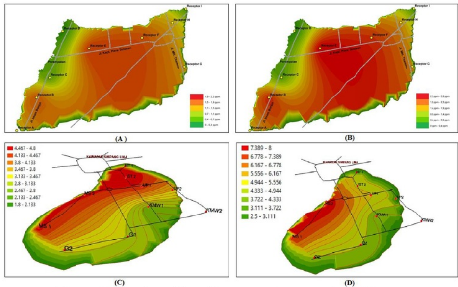
Figure 4. Increasing ambient CO concentration surrounding CFD area.
