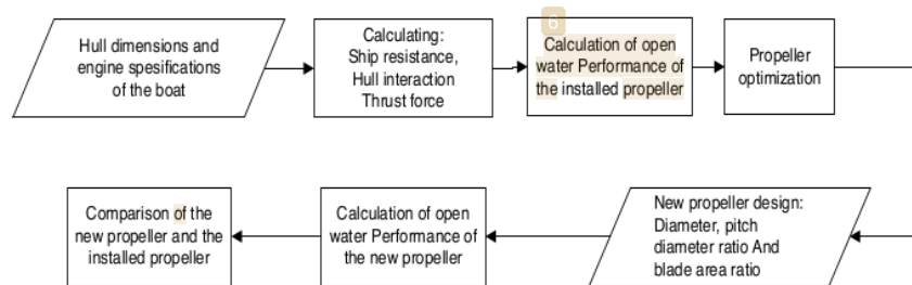
Figure 2 Flowchart of the B-Series propeller design and optimization using free software.
