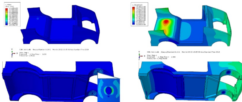
Gambar 4 sample hasil simulasi FEM chassis kasus 1 material aluminium AISI 6061.
