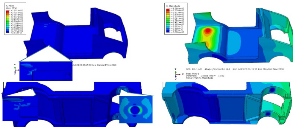
Gambar 5 sample hasil simulasi FEM chassis kasus 1 material carbon fiber.
