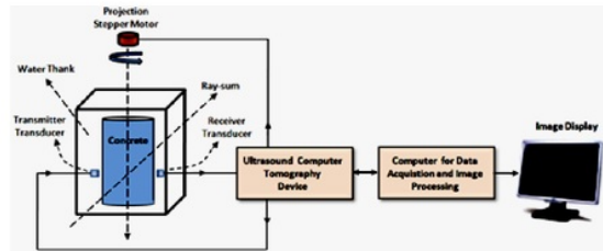
Figure 3. Experimental scheme of the ultrasound computer tomography
