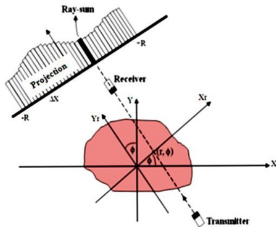
Figure 1. Scanning process in ultrasound tomography
