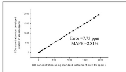
Fig. 5. Calibration result of the CO concentration measurement instrument.
