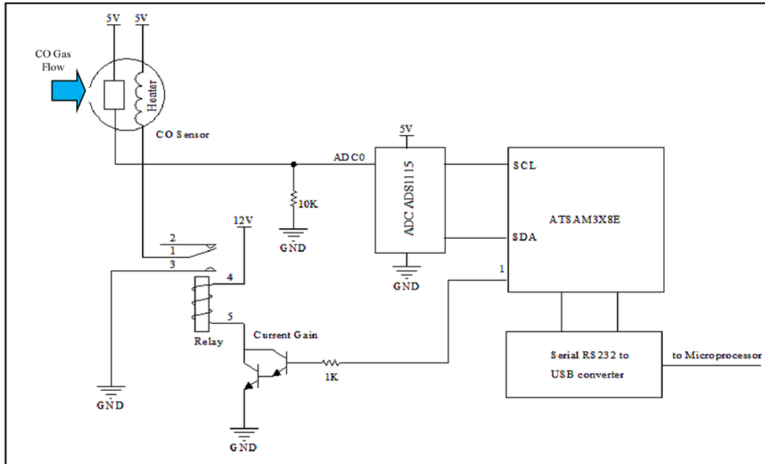
Fig. 2. A Carbon monoxide sensor and interface circuit.
