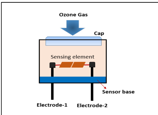
Fig. 2. Construction of an ozone sensor.
