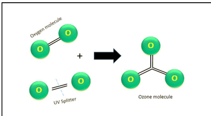
Fig. 1. Chemical reaction resulting in ozone formation.
