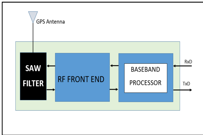
Fig. 4. Architecture of GPS module.
