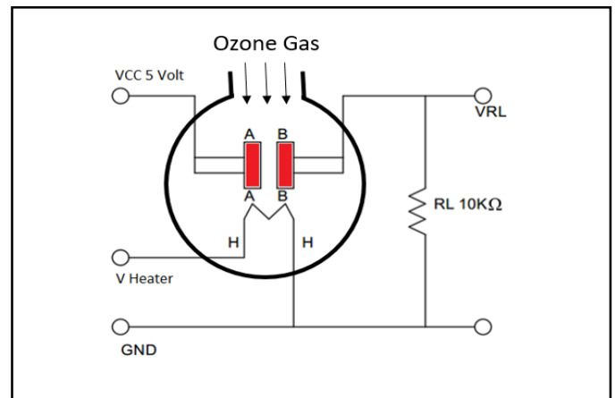
Fig. 3. Construction and circuit of an ozone sensor.
