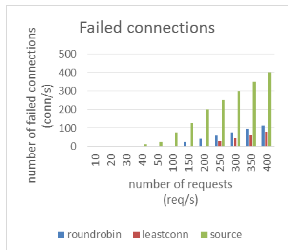
Fig. 7. Failed connections of every algorithm in scenario (2)
