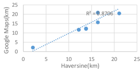
Fig. 6. RMS between Google Maps and Haversine
