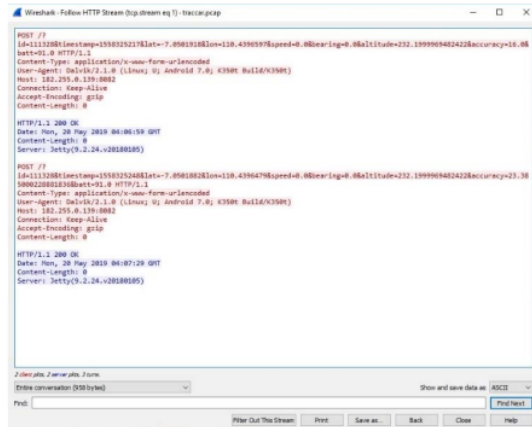
Fig. 3. Wireshark analysis of GT-06A POST parameter
