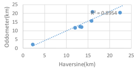
Fig. 5. RMS between Odometer and Haversine
