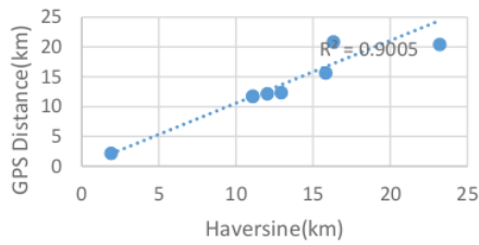
Fig. 7. RMS between GPS distance and Haversine
