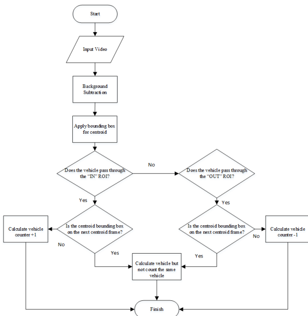
Fig. 5. Flowchart of vehicle calculation at parking space
