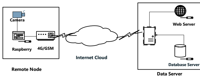
Fig. 1. The designed system in IoT architecture
