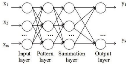
Fig. 1. Architecture of the GRNN model
