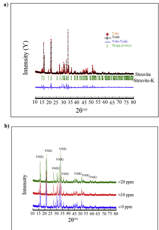
Figure 3. a) XRPD Rietveld refinement plot of the precipitates in the solution at 30 °C without maleic acid; b) XRPD patterns of all samples with 0, 10, and 20 ppm maleic acid. The peaks are labelled S (struvite); S(K) (struvite-K).
