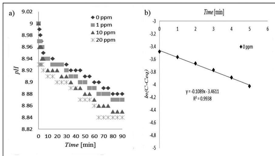
Figure 1. Struvite crystallization at 30 °C with and without maleic acid; (a) pH reduction profile; (b) fit of first order kinetic without maleic acid. C = [\text{Mg}^{2+}] at time t ; C_{eq} = [\text{Mg}^{2+}] at equilibrium, i.e. when the crystallization was completed.
