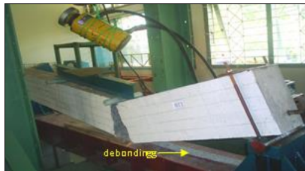
Figure 13. Beam with CFRP failed through debonding mechanism
