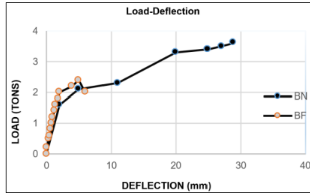
Figure 14. Comparison between load versus deflection between BN and BF
