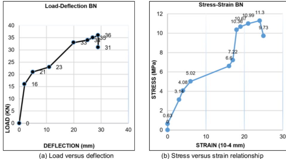
Figure 10. Load–deflection and stress–strain for normal beam (BN)
