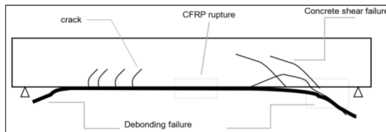
Figure 6. The mechanism of rupture in the beam given CFRP (Kuriger et al., 2001)
