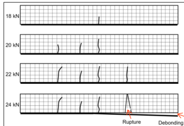
Figure 16. Cracks Pattern of BF
