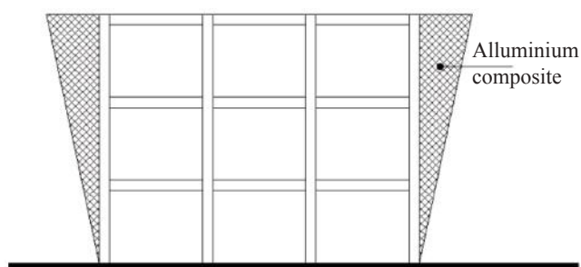
FIGURE 8. Weak story due to reversed pyramid form can be minimized by using flexible and light materials like aluminum composite
