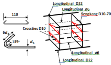
Gambar 1. Detail crosssties
