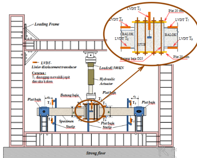
Gambar 4. Set up pengujian (Priastiwi et al. , 2017)
