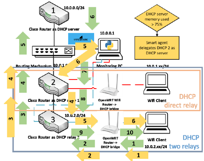
Fig. 5. Examination The proposed Smart Agent and DHCP relays when DHCP relay 2 handles the job of DHCP server.
