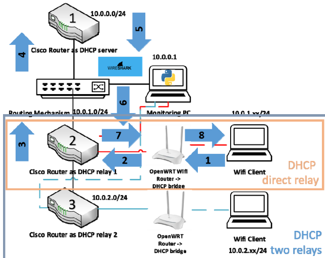
Fig. 2. Overall system in the default scenario in Cisco environment.
