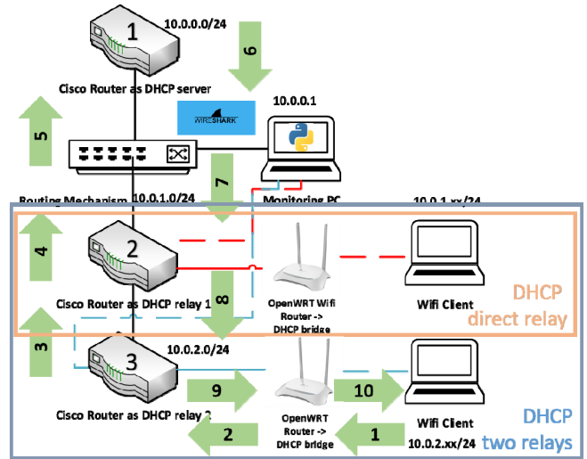
Fig. 4. Examination scenario of the proposed smart algorithm using two DHCP relays.
