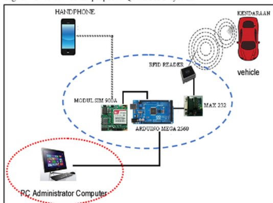
Fig. 1. Overview of the proposed Queen ATG system.
