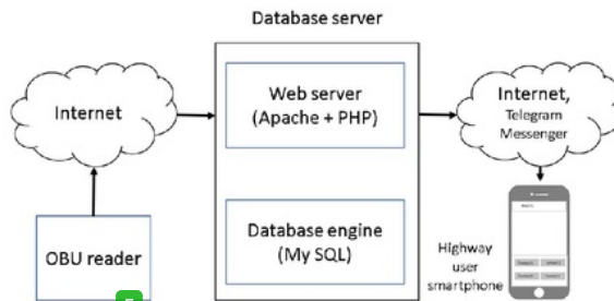
Fig. 7. Block diagram of the data processing part.
