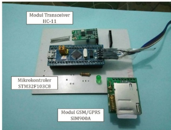
Fig. 6. OBU reader, installed in toll gate consists of Microcontroller STM32F103C8, Transceiver module HC-11 to receive data from OBU, and GSM/GPRS module SIM900A to send data to the Internet.
