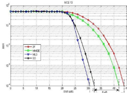
Fig. 1. Performance comparison of ZF, MMSE, MLD, and SD for MCS 13 of WLAN 802.11n 40MHz.
