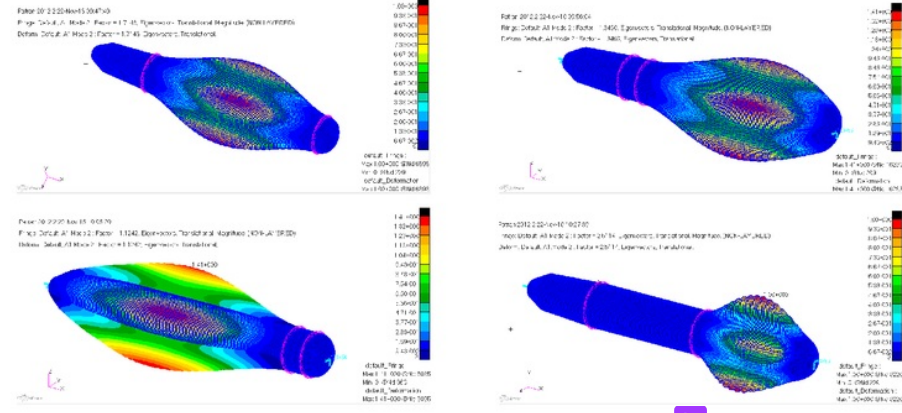
Figure 3 2 nd mode buckling mode shape: [a] model 1; [b] model 2; [c] model 3; [d] model 4
