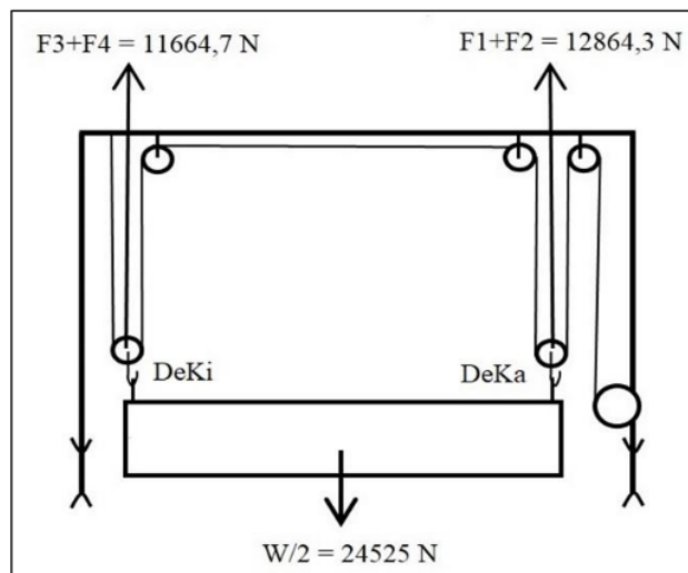
Figure 7. The Difference of Lifting Forces
