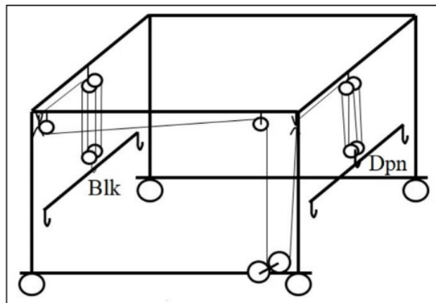
Figure 5. The 8/2/2/1+Spreader-DeBe System
