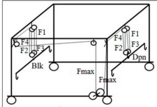
Figure 8. Synchronous Lifting System
