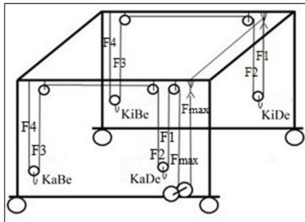
Figure 6. The Lifting Force of Existing System
