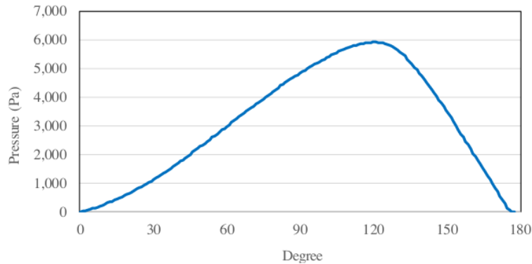
Gambar 5. Grafik distribusi tekanan synovial fluid
