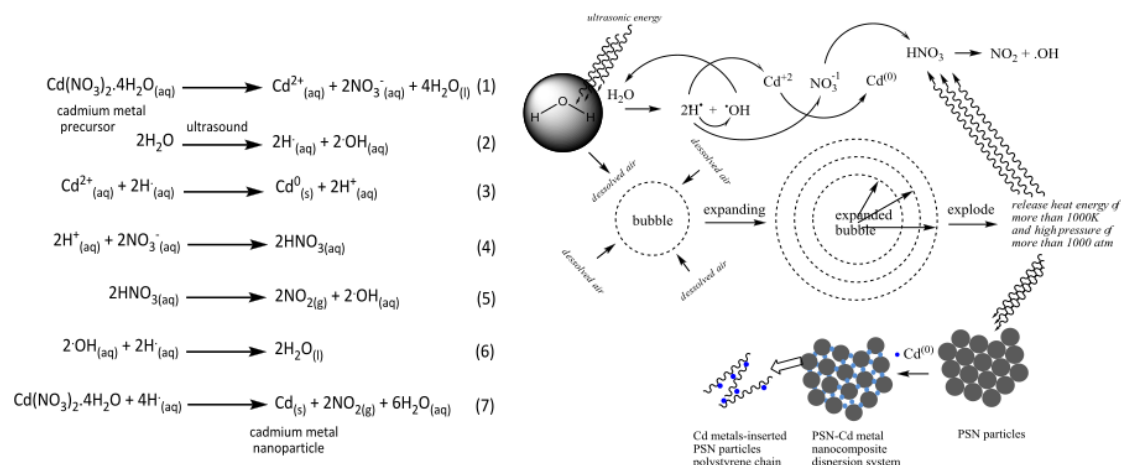
Figure 3. Schematic illustration of the reduction reactions of \text{Cd}^{2+} through "hot spots" mechanism generated by ultrasonic irradiation of 40 kHz for 45 minute.
