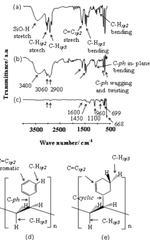
Figure 4. ATR-FTIR spectra of pristine PSNs (a), composite material of PSNs/CdMNp (b), and Laser-exposed composite material of PSNs/CdMNp (c). These spectra were adopted from reference [13] for spectra (b) and (c). Illustration of Polystyrene molecular structure unit (d) and (e).
