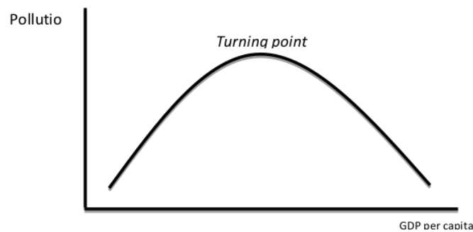
Figure 2. Environmental Kuznets Curve (EKC)
