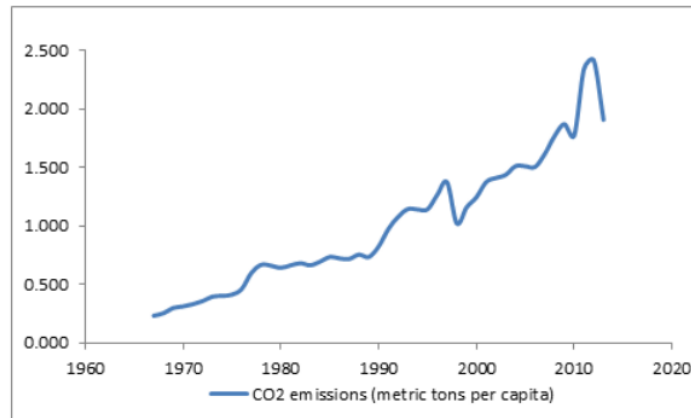
Figure 1. Trend of CO2 Emission of Indonesia of 1967-2013
