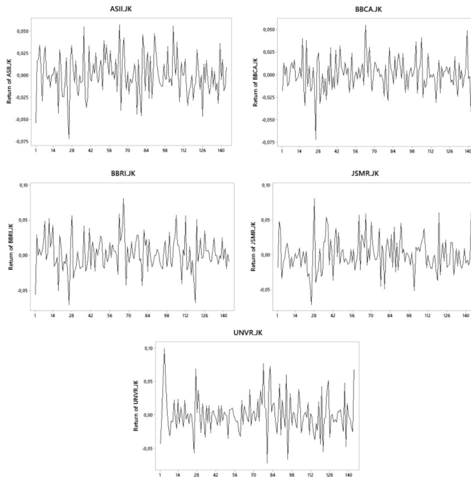
Figure 2 TIME SERIES PLOT OF IN SAMPLE RETURN
