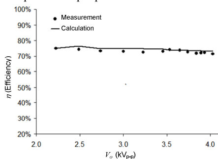
Fig. 9. Efficiency of Circuit-3
