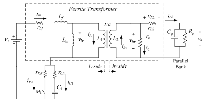
Fig. 2. Schematic circuit for resonant converter with ferrite transformer.
