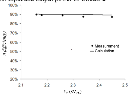
Fig. 7. Efficiency of Circuit-2
