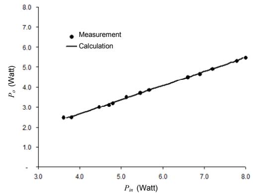
Fig.4. Input and output power of Circuit-1
