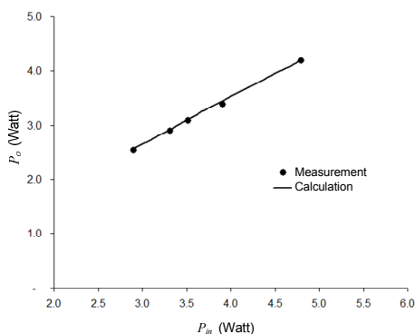
Fig. 6. Input and output power of Circuit-2
