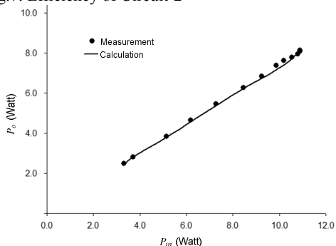
Fig. 8. Input and output power of Circuit-3
