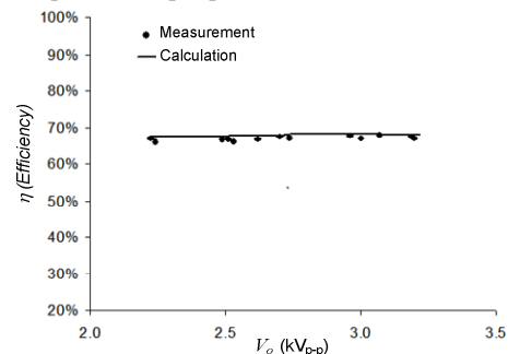
Fig.5. Efficiency of Circuit-1
