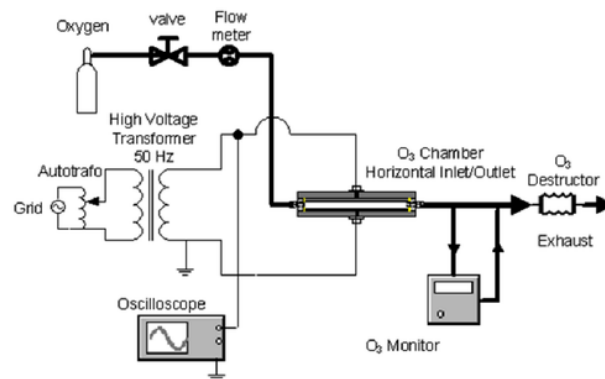
Figure 3. The experimental set up with 50 Hz AC supply
