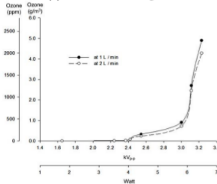
Figure 11. Ozone Concentration in ppm as a function of applied voltage in Volt
