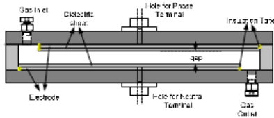
Figure 1. Ozone chamber
