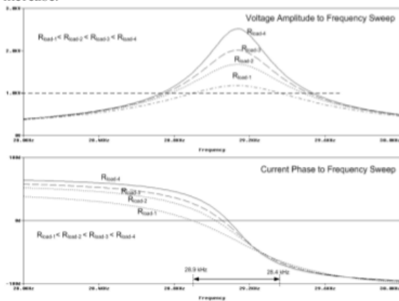
Figure 8 Simulation Result of Frequency Sweep Program
