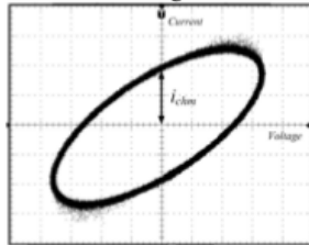
Figure 2. I-V characteristics in Lissajous Pattern
