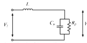
Figure 5. Equivalent Circuit of Ozone Chamber as part of Parallel Loaded Resonant Circuit
