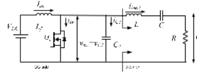
Figure 4. Fundamental Circuit of Single Switch Resonant Converter
