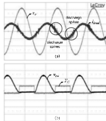
Figure 10.a Output voltage at terminal chamber Voltage (500V/div) and Current (50mA/div) at chamber side; 10.b. control signal, V_{sw} (20 Volt/div) and voltage at low voltage side, V_C (50V/div)
