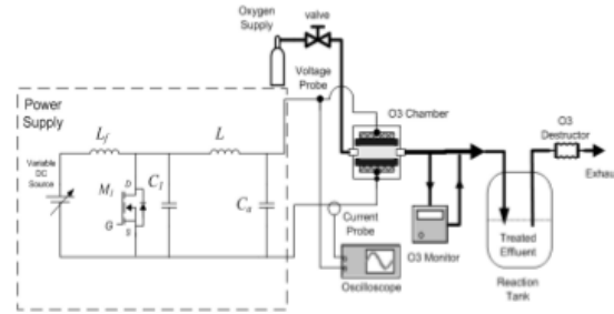
Figure 9. Experimental Set Up of ozonizer for Colour Removal
