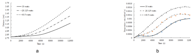
Figure 4: Distance rate at various power supply (a) and evaporation rate at various power supply (b)
