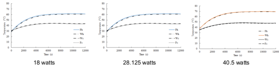
Figure 3: Temperature as a function of time and power supply
