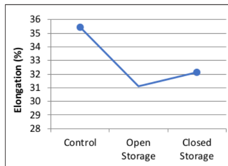
Figure 4. Elongation average graph
