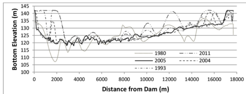
Fig. 6. Longitudinal Profil of Bengawan Solo River
