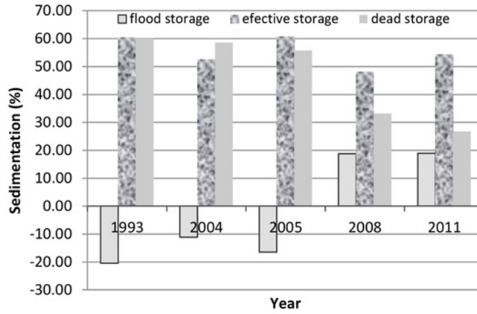
Fig. 3. Sediment deposition in each zone for year 1993 - 2011
