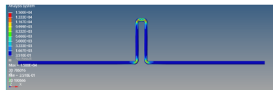
Figure 4: Stress occurring in the expansion loop pipe.
