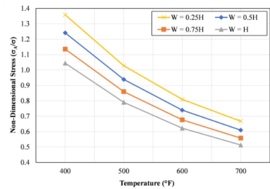
Figure 11: Relationship between \sigma_A/\sigma on the expansion loop pipe 24-inch diameter with increasing temperature.
