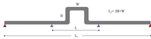
Figure 1: Symmetrical Expansion Loop.
