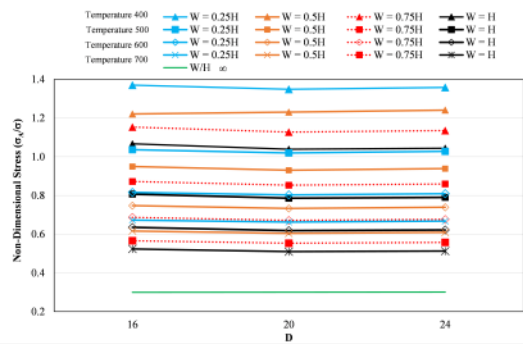
Figure 13: Relationship between \sigma_A/\sigma with the pipe diameter (inch).
