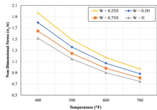
Figure 12: Relationship between \sigma_y/\sigma on the expansion loop pipe 24-inch diameter with increasing temperature.
