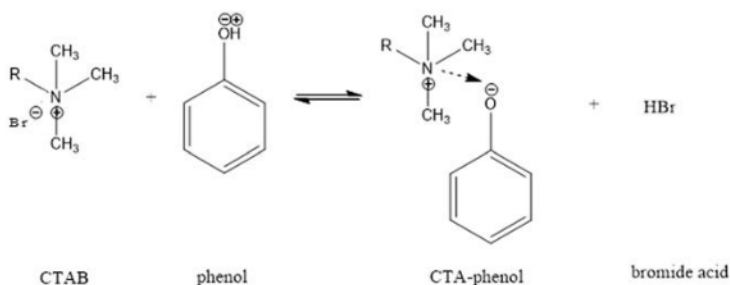
Figure 5: Reaction scheme between CTAB and phenol.
