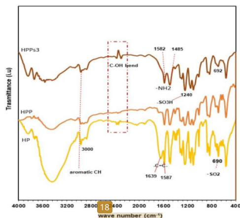
Figure 1. FTIR spectra of the membranes
