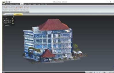
Figure 6. Combination of TLS and UAV Point Clouds
