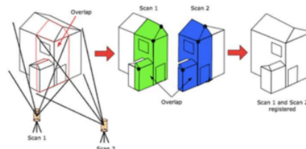
Figure 1. Illustration of cloud to cloud method
