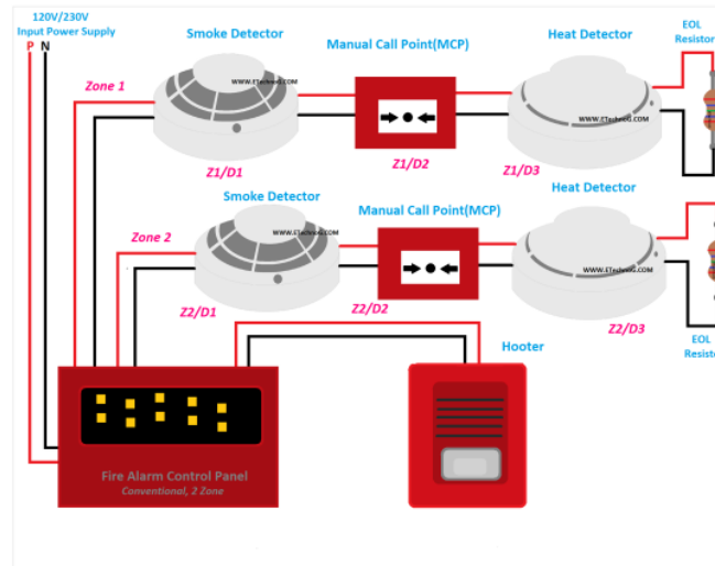
Fig. 1. A typical fire alarm system wiring diagram.
