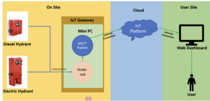
Fig. 3. Architecture of the IoT-based FSS monitoring system.
