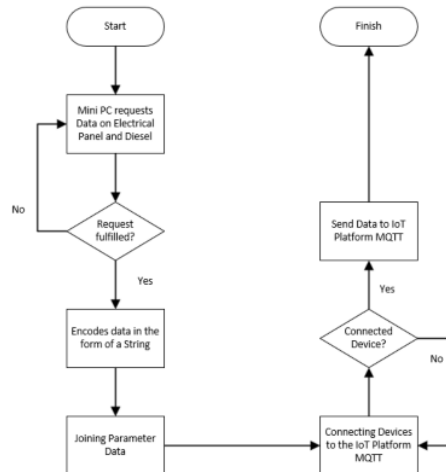
Fig. 4. Flowchart of the IoT-based FSS monitoring system.
