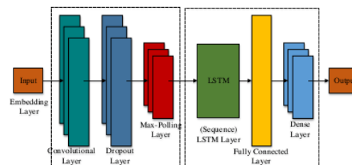
Figure. 3 CNN-LSTM architecture for training data
