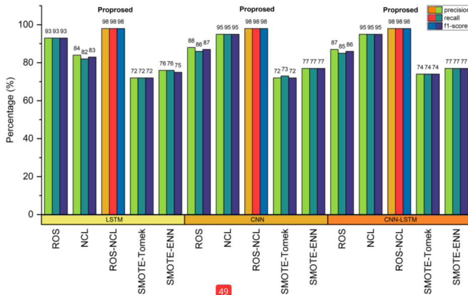
Figure. 6 Average precision, recall, and F1 score
