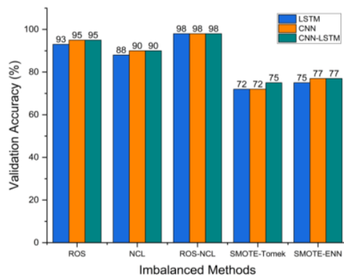
Figure. 7 Validation of the accuracy
