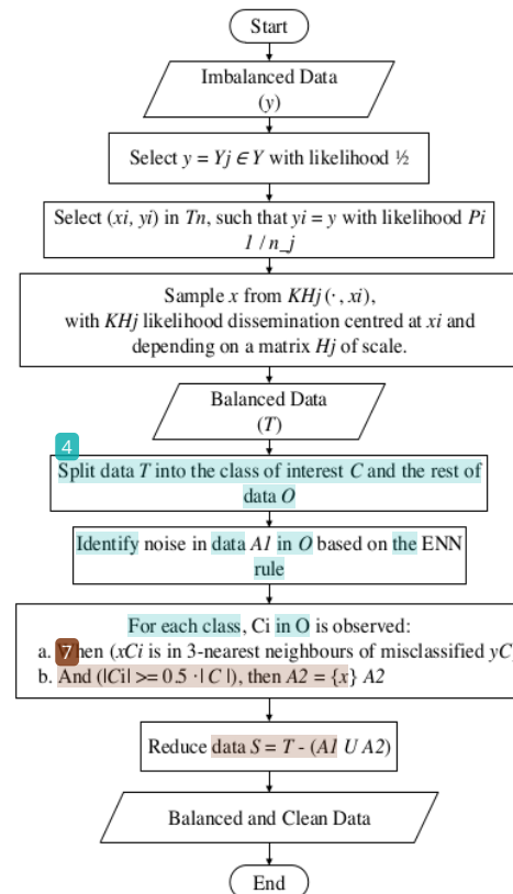
Figure . 2 The Proposed hybrid sampling ROS-NCL method
