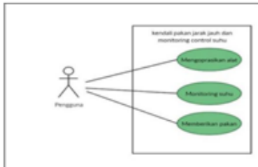
Gambar 1 Use Case
