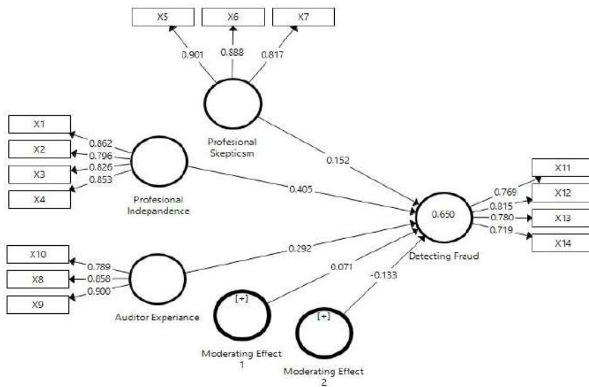
Figure 3. Structural Model of External Auditors
