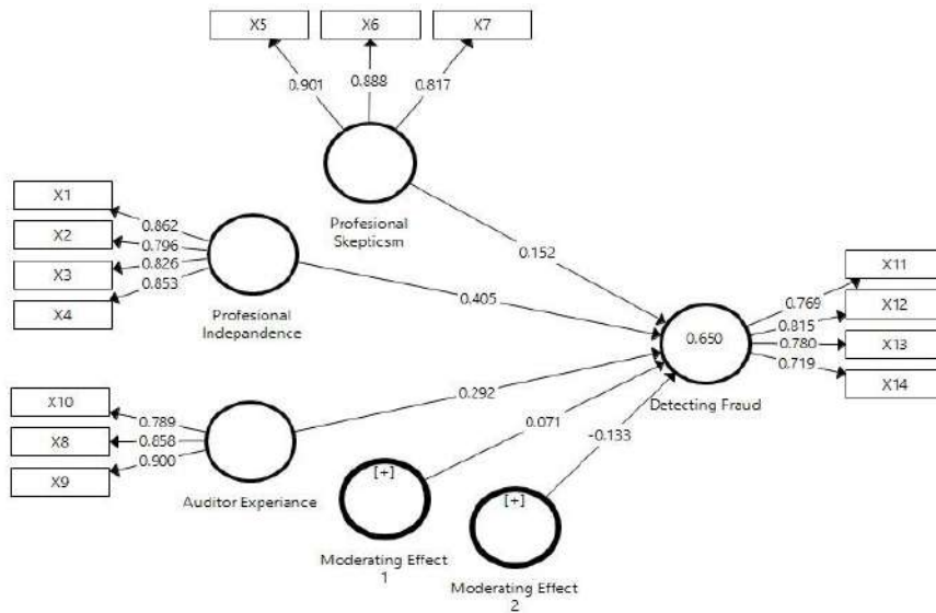
Figure 3. Structural Model of External Auditors
