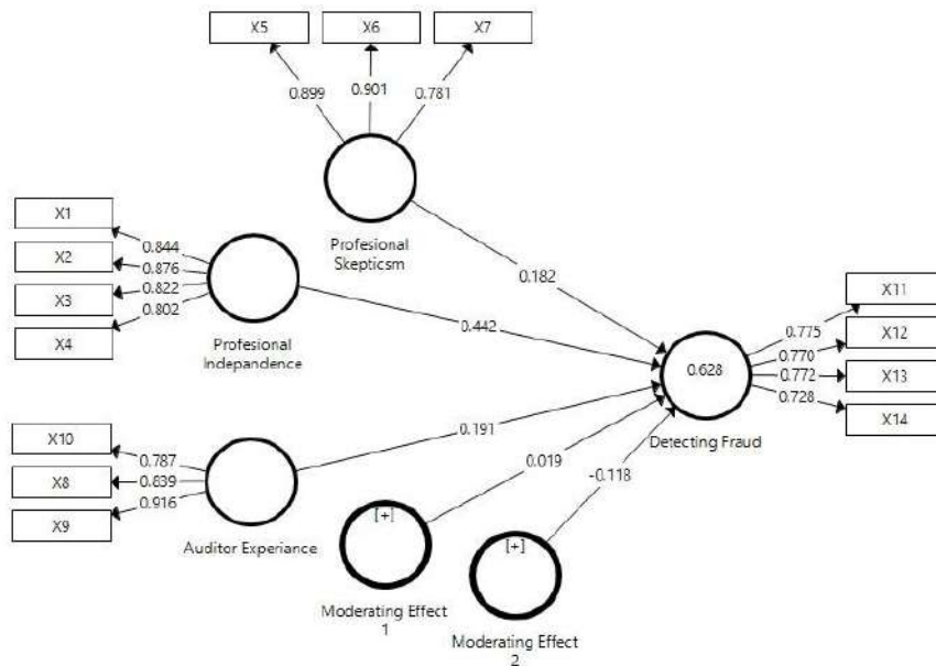
Figure 2. Internal Auditor Structural Model
