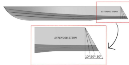
Figure 2. Extended stern variations.
