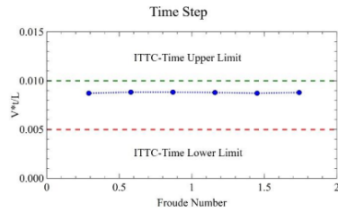
Figure 5. Time-Step.
