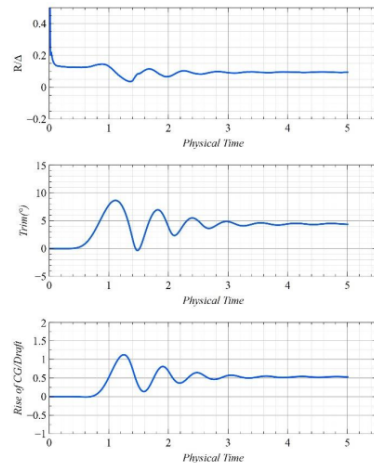
Figure 8. The convergence of hydrodynamic characteristics in time.
