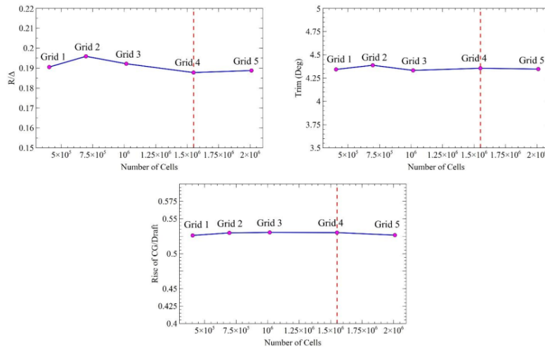
Figure 7. Grid independence of drag, trim, and heave.
