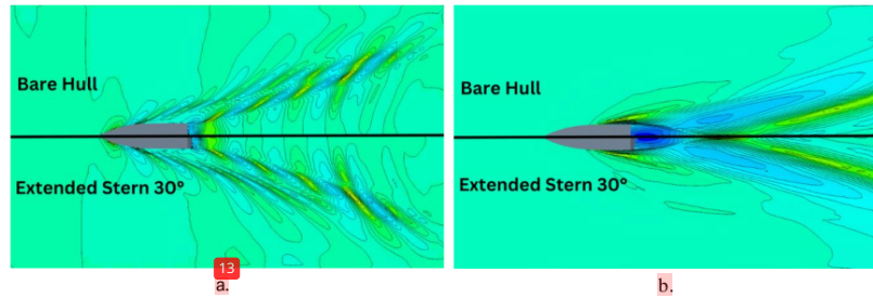
Figure 11. Wave pattern (a) Fr 0.29 and (b) Fr 1.16.
