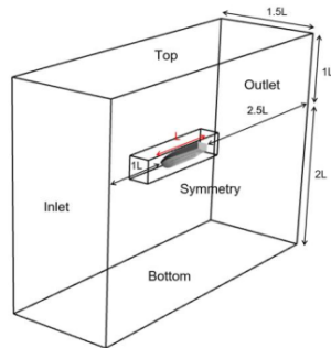
Figure 3. Computational domain and boundary condition.
