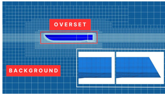
Figure 6. Mesh Density.
