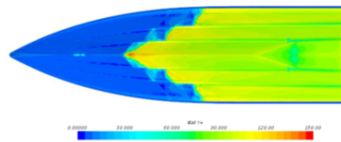
Figure 4. Wall y^+ .
