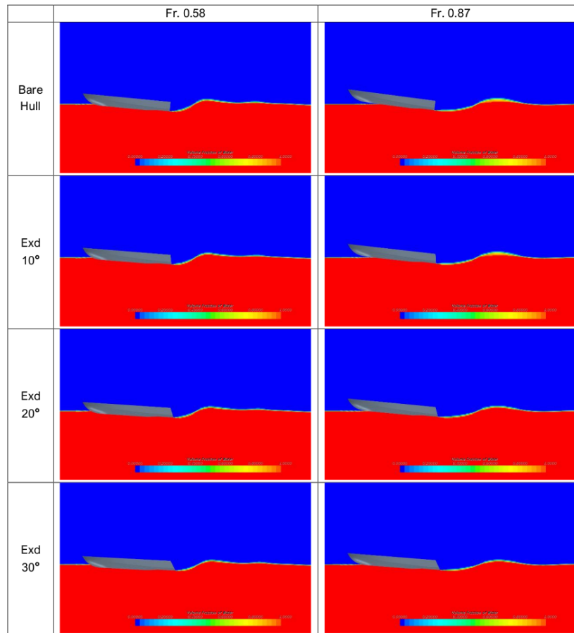
Figure 12. Visualization of trim on Froude number 0.58 and 0.87.
