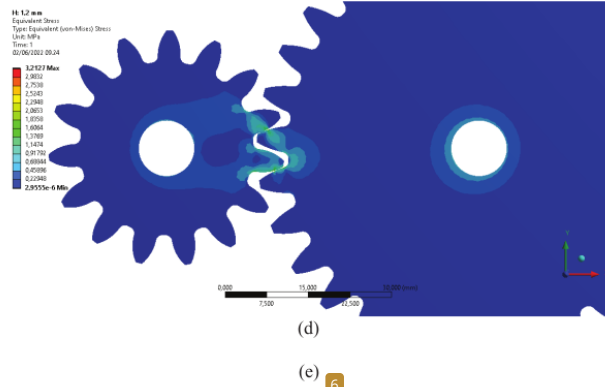
FIGURE 4. Stress generated on various fillet radius spur gear (a) 0.9 mm; (b) 1 mm; (c) 1.1 mm; (d) 1.2 mm; (e) 1.3 mm
