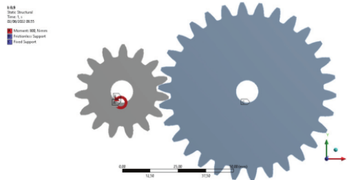
FIGURE 2. Boundary condition
