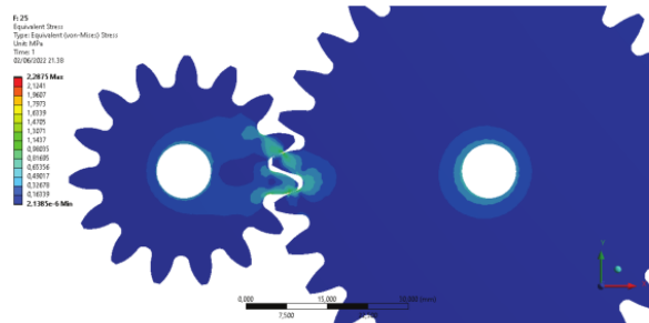
FIGURE 5. Von Misses Contour of the Optimized Plastic Gear.
