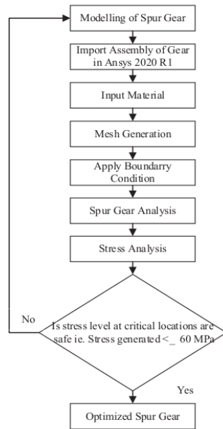
FIGURE 3. Flowchart of shape optimization plastic gear
